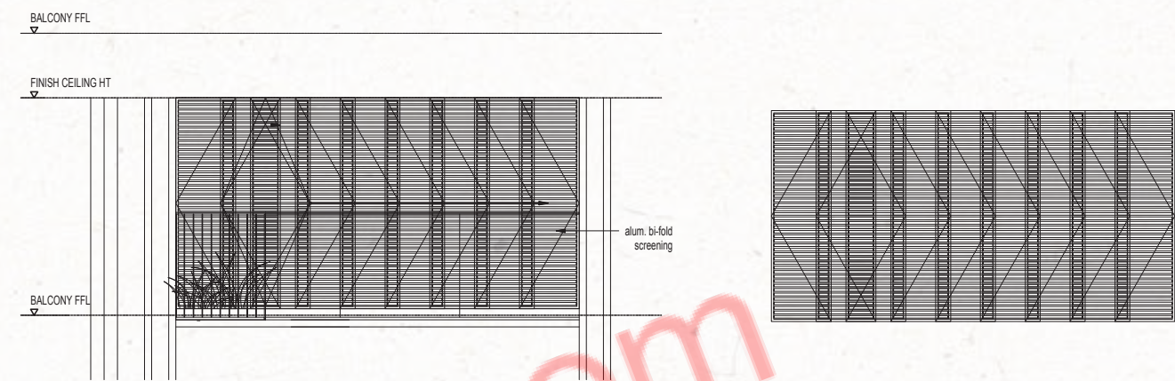
TYPICAL ELEVATION OF BALCONY WITH SCREEN
