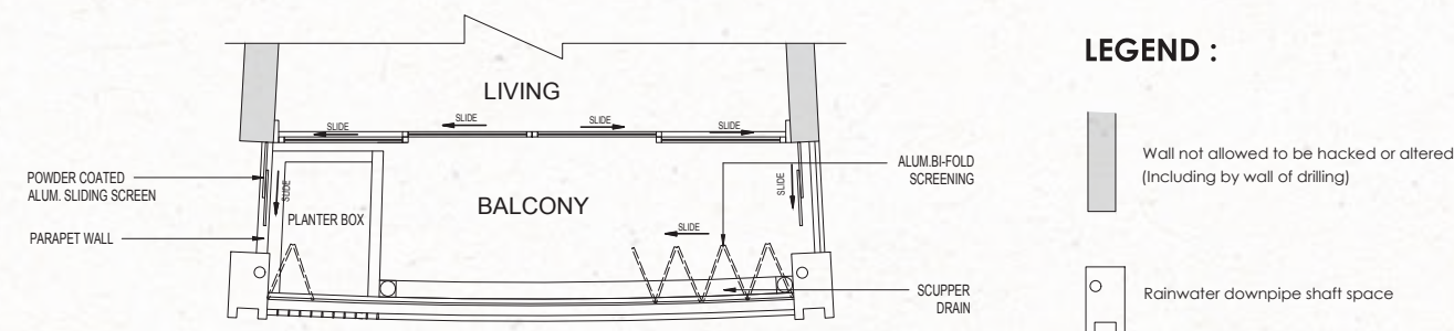
TYPICAL PLAN WITH BALCONY SCREEN
