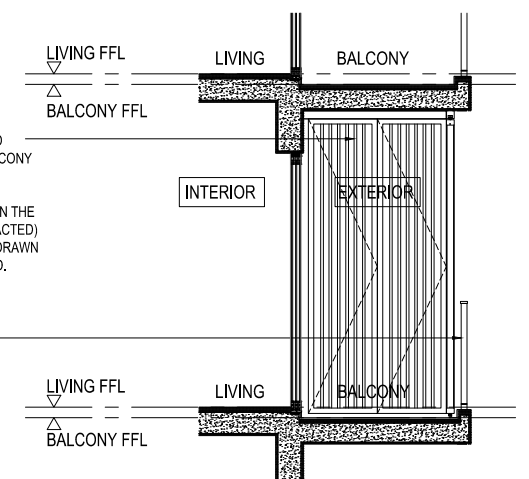
SECTION
